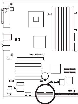
P5GDC PRO Floppy disk drive connector
